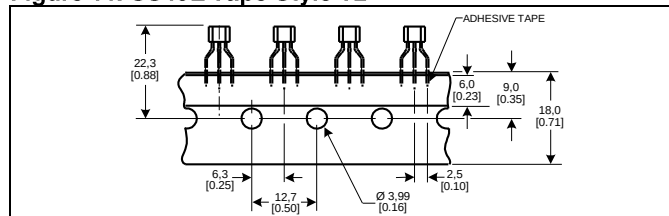
Figure 11. SS49E Tape Style T2
