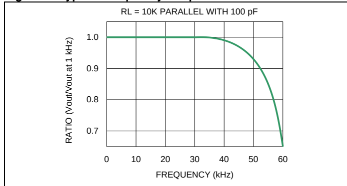
Figure 5. Typical Frequency Response
