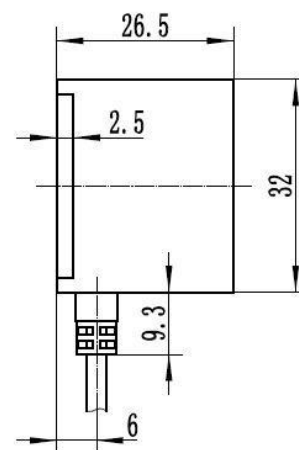
Figure 2. Top view of HPS-167U
