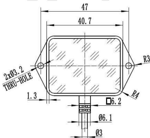
Figure 1. Front view of HPS-167U
