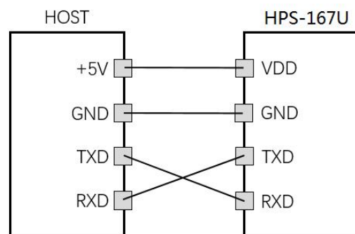
Figure. 3 Application schematic of the HPS-167U
