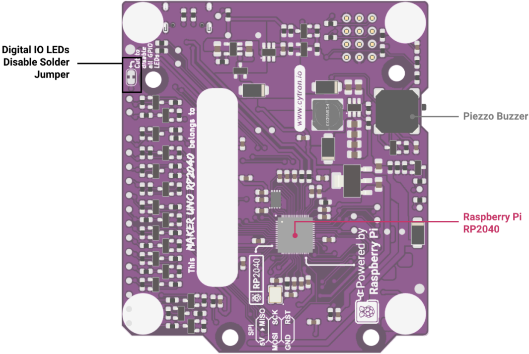
Figure 2: MAKER-UNO-RP2040 Board Functions (Bottom)
