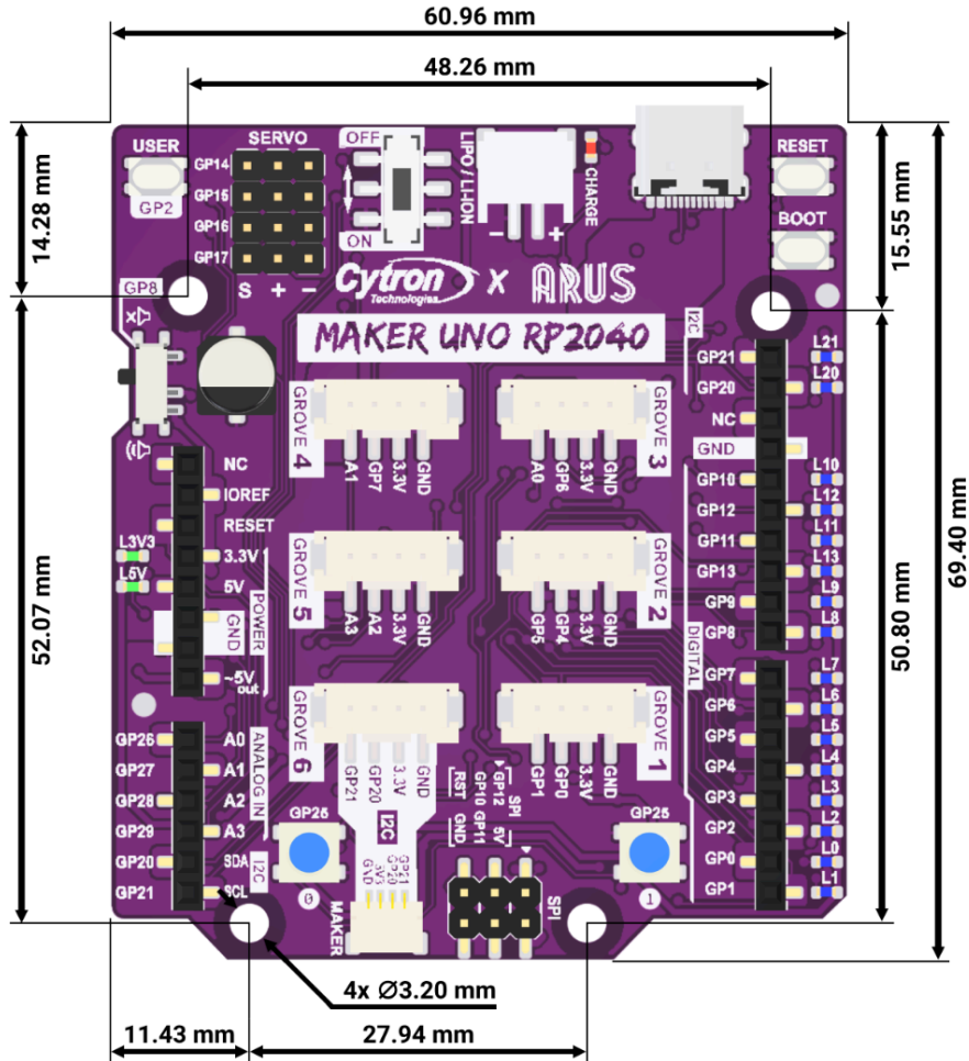
Figure 4: MAKER-UNO-RP2040 Dimension
