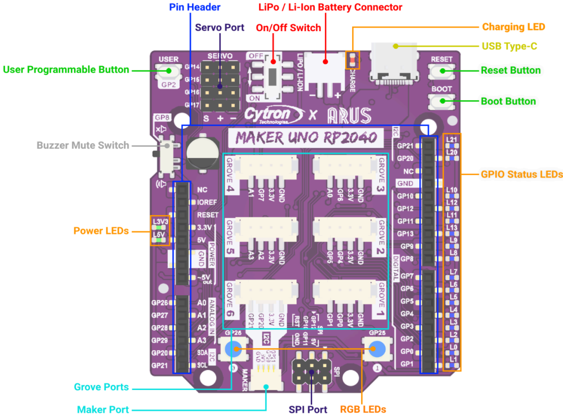
Figure 1: MAKER-UNO-RP2040 Board Functions (TOP)
