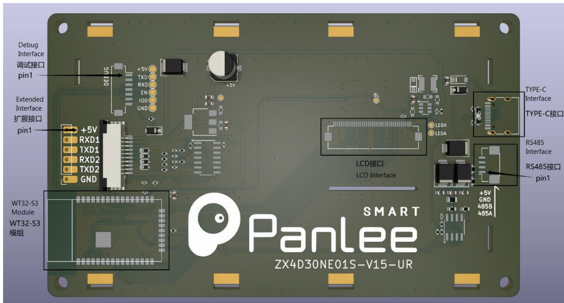
Fig. 1 Hardware Interface
